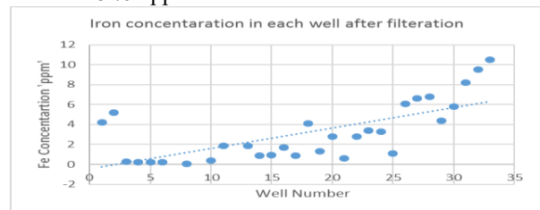
Fig. 4: Iron concentration in each well after omitted the three wells
