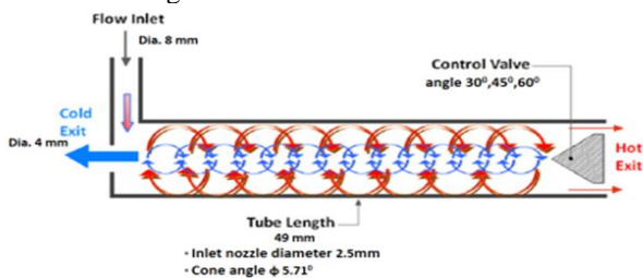
Fig.2: Schematic diagram of Vortex Tube
