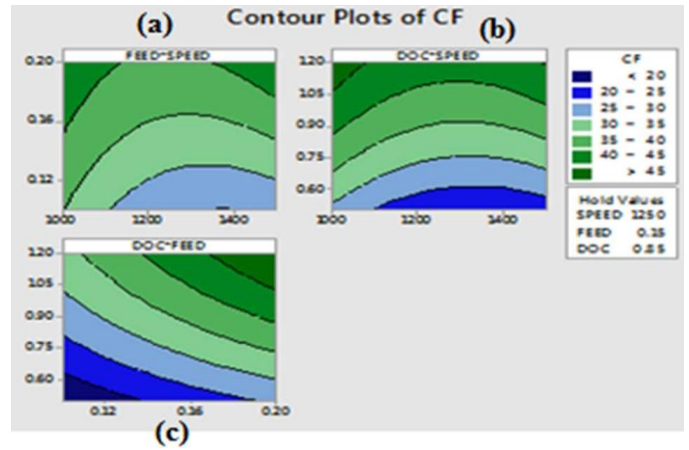
Fig 9: Contour plot represents relation between speeds, feed, Doc ad CF
