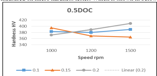
Fig: 5 Hardness variation with cutting speed for a depth of cut 0.5mm at various feed
