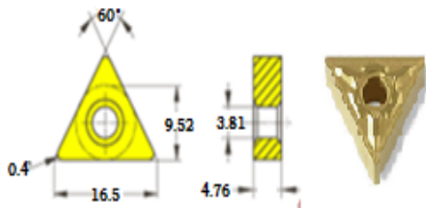
Fig 1 Cutting Tool Insert dimensions.
