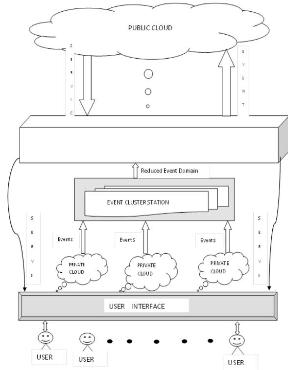
Fig-2: Event Reducing Model
