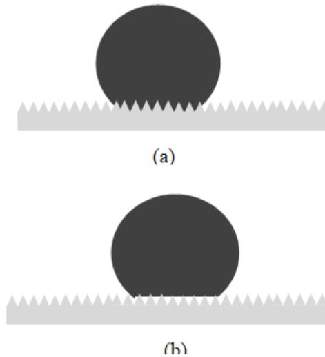
Fig2 (a) Homogeneous wetting on hydrophobic ( \theta_y>90^\circ ) surface; Wenzel model [2] (b) Inhomogeneous wetting on hydrophobic ( \theta_y>90^\circ ) surface) Inhomogeneous wetting on hydrophobic ( \theta_y>90^\circ ) surface; Cassie-Baxter model [3]
