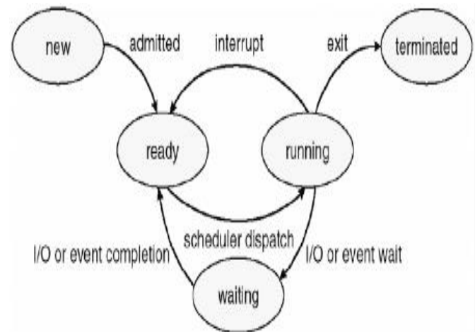
Figure 1 Process scheduling
