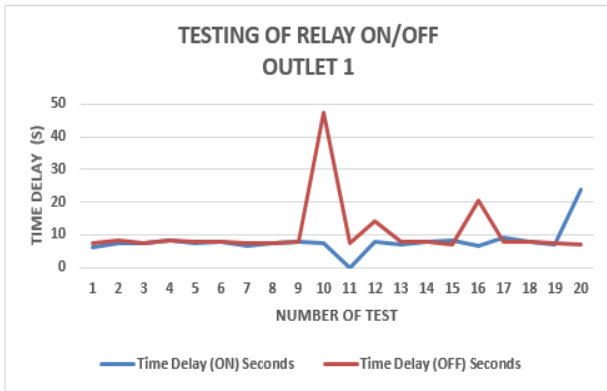
Figure 7: Relay (ON/OFF) Testing on Outlet 1 with an Electric Fan
