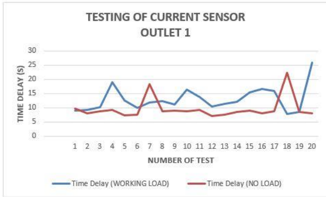
Figure 9: Current Sensor Testing on Outlet 1 with an Electric Fan
