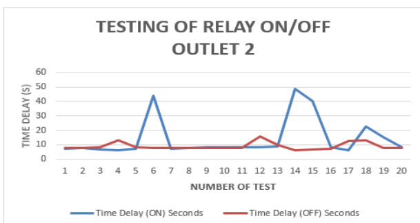
Figure 8: Relay (ON/OFF) Testing on Outlet 2 with an Electric Fan
