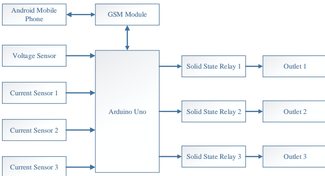
Figure 2: Systems Block Diagram
