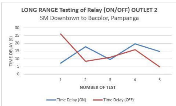
Figure 12: Relay response (ON/OFF) testing in long-range for Outlet 2
