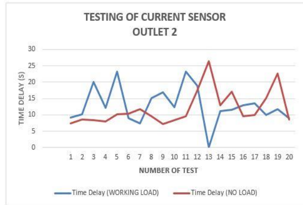
Figure 10: Current Sensor Testing on Outlet 2 with an Electric Fan
