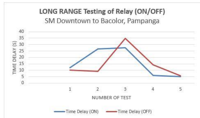
Figure 11: Relay response (ON/OFF) testing in long-range for Outlet 1
