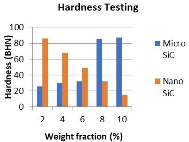
Figure 6: Effect of Micro & Nano Sized Silicon Carbide on Hardness
