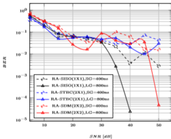
Fig 5. BER v/s SNR over TGn C channel with NLOS
