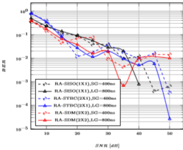
Fig 3. BER v/s SNR over TGn B channel with LOS
