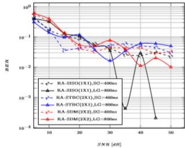
Figure 7. BER v/s SNR over TGn D channel with NLOS
