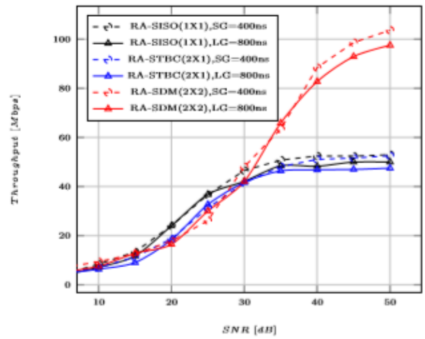
Fig 6. Throughput v/s SNR over TGn D channel with NLOS
