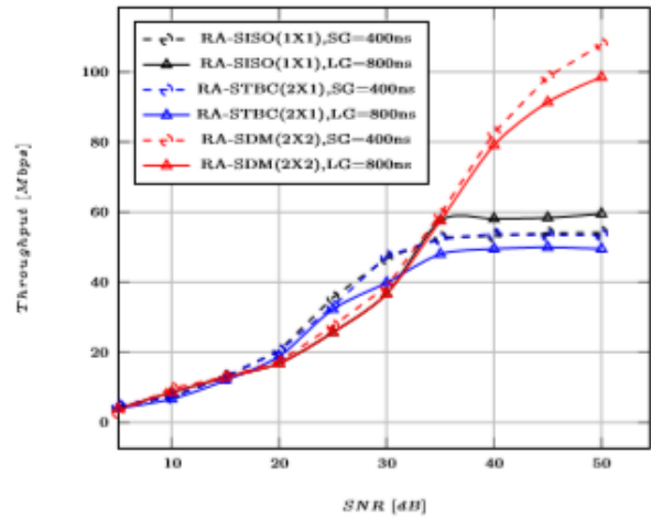
Fig 2. Throughput v/s SNR over TGn B with LOS
