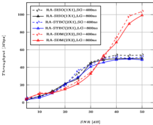
Fig 4. Throughput v/s SNR over TGn C channel with NLOS
