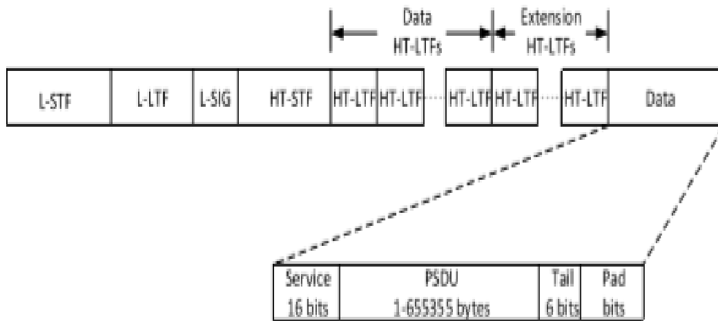
Fig 1. HT-mixed packet structure
