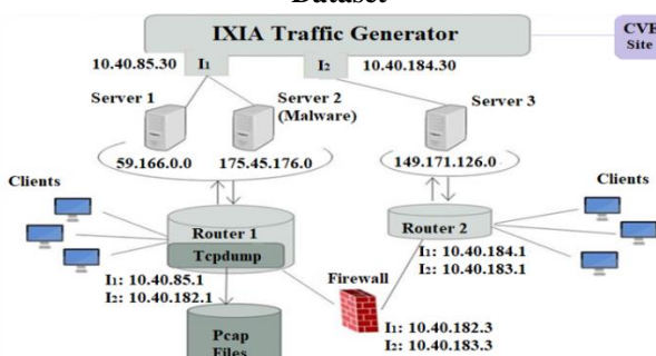
Fig.2: UNSW-NB15 Testbed
