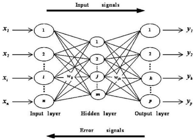
Fig. 1. Three-layer NN [4].
