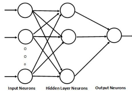
DC-ELM architecture
