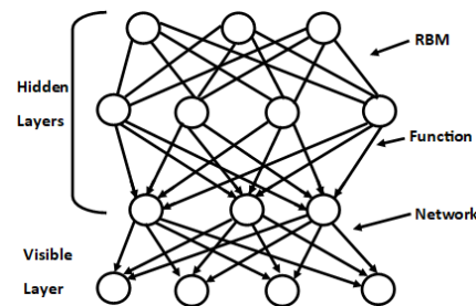
Fig 6. DBN Architecture
