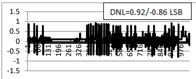
Fig 11 Simulated DNL
