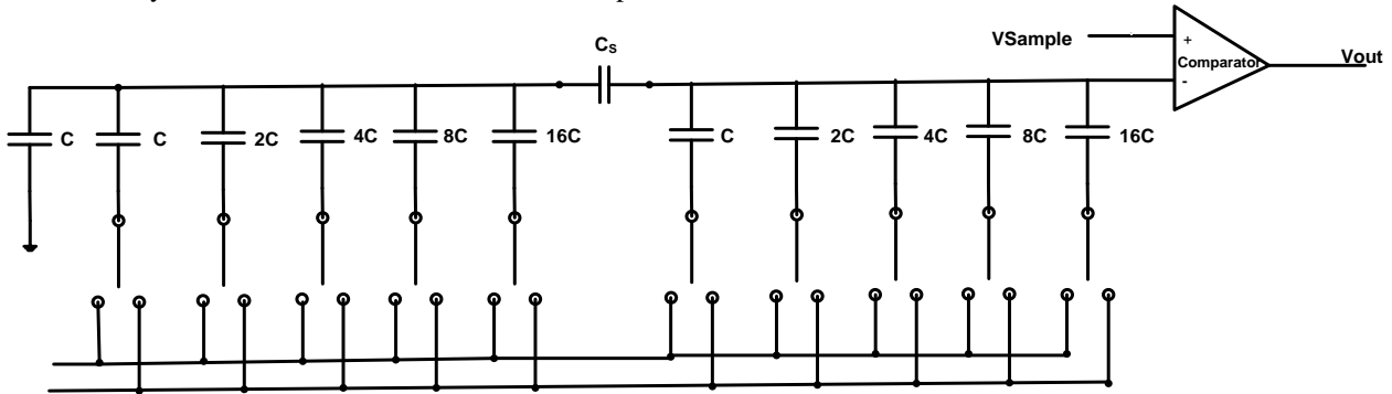
Fig.3 Charge scaling 10 bit Digital to Analog Converter
