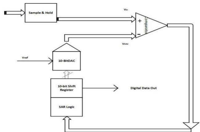
Fig 1 Design of SAR ADC
