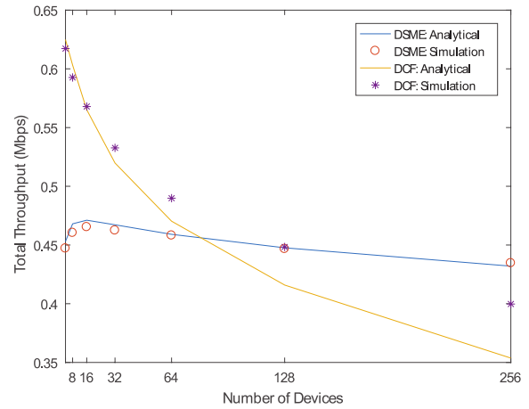
Fig. 2 Throughput for various devices
