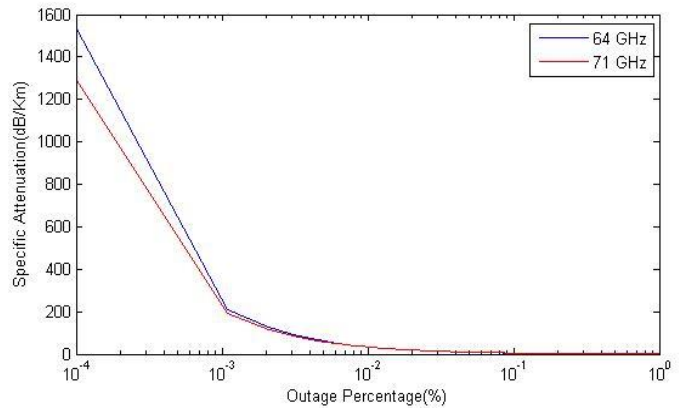
Fig. 6: For 64-71 GHz
