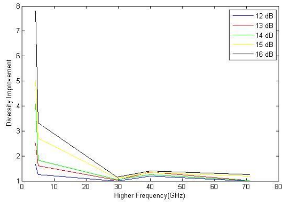
Fig.7. Correction factor for aforesaid frequency ranges in frequency variation scheme
