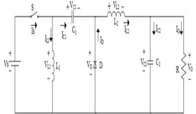
Fig5. Circuit diagram of voltage lift Luo Converter
