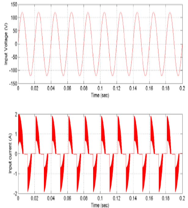
Fig10. Simulation outputs depicting input voltage and current waveform
