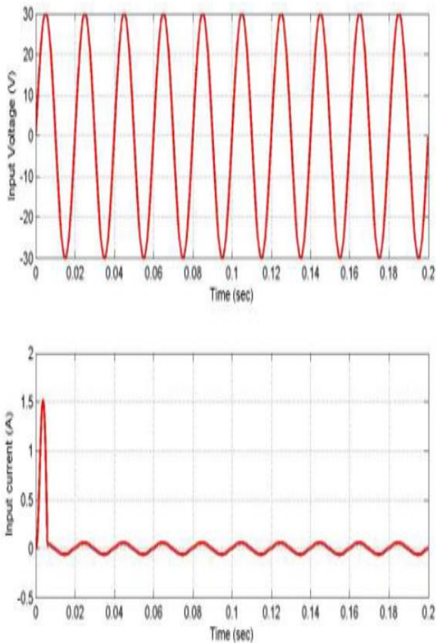
Fig8. Input current of proposed system
