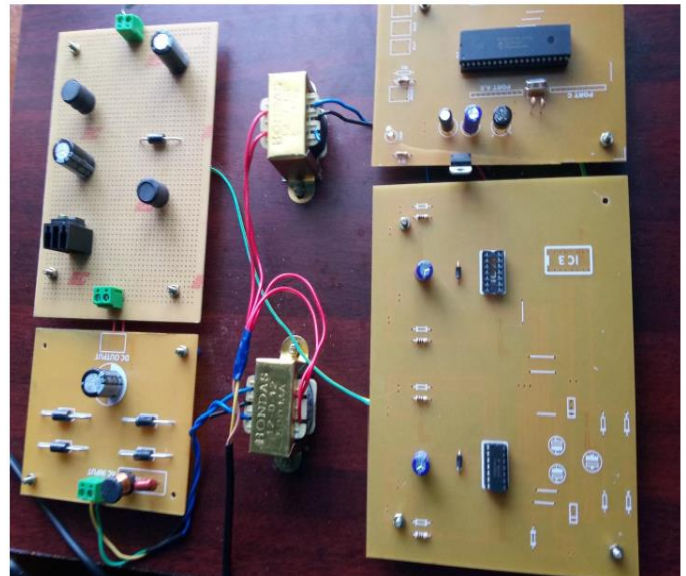
Fig13. Hardware implementation of the topology
