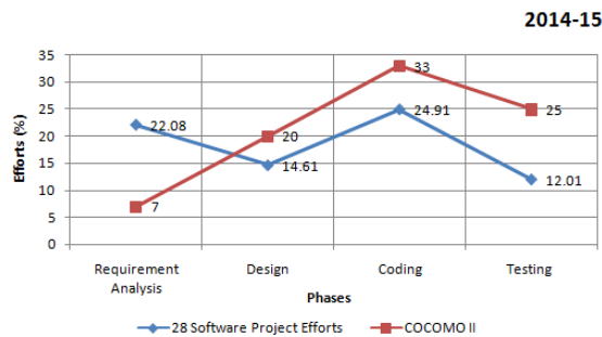
Fig. 1(a). Comparison of 28 software projects with COCOMO II model (Waterfall Distribution Magnitude) for academic year 2014 – 15
