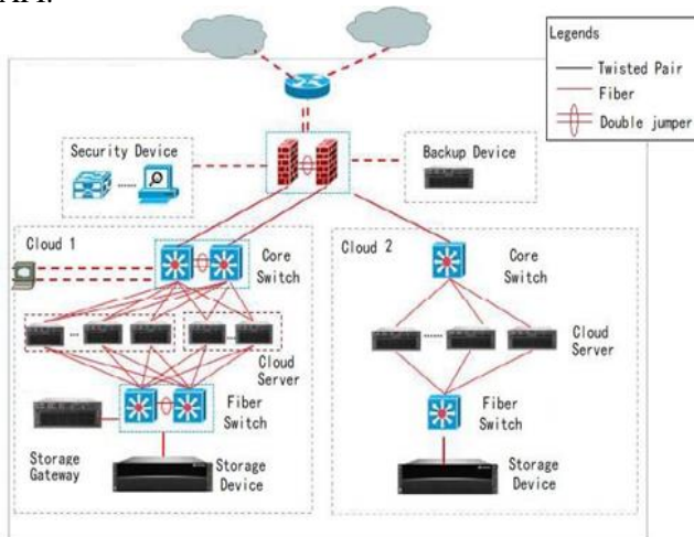
Fig. 5. Experimental Environment for Cloud Security Computable Assessment
