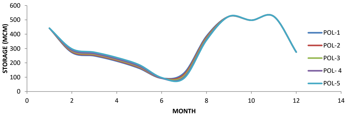
Fig. 7 End month storages under 50% dependable inflow
