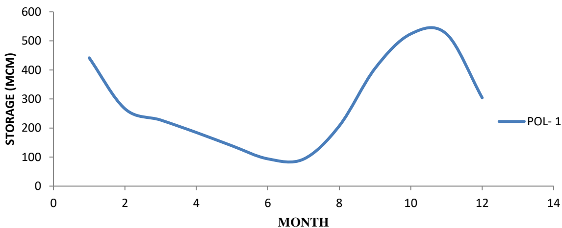
Fig.9. End month storage under 90% dependable inflow.
