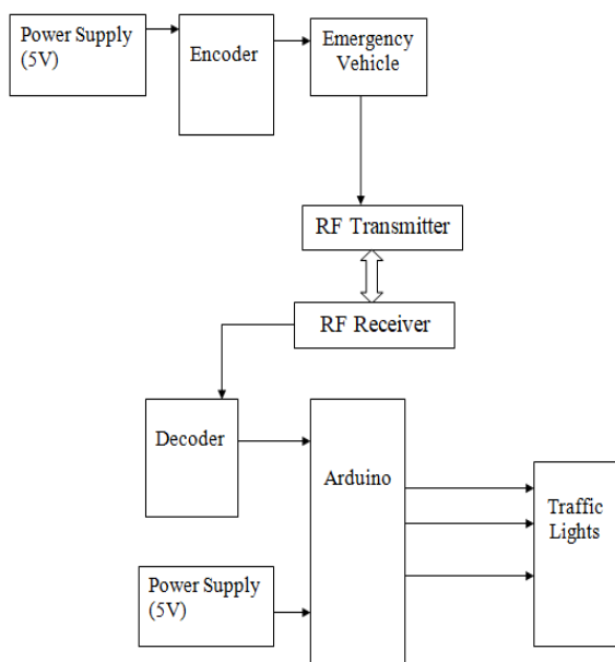
Figure 1. Block Diagram of Traffic Controlling System for Emergency Vehicle
