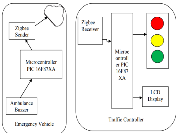
Figure 6. Efficient Way of Traffic Control System
