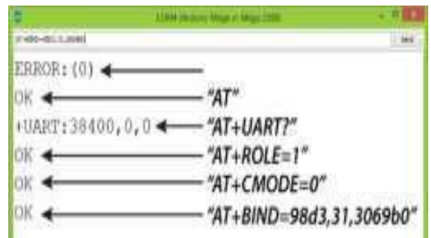
Figure 6 Configuration for the Bluetooth module as a Slave
