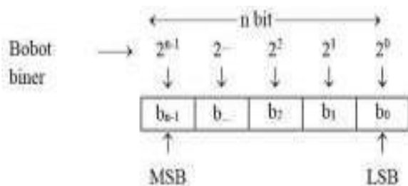
Figure 3 Representation of Binary Integers
