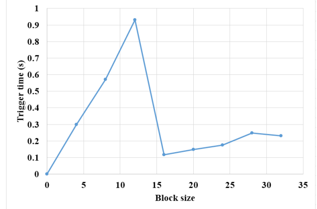
Figure 2. Trigger time of the proposed ECDSA method with various block size
