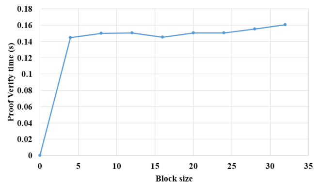
Figure 3. Proof verify time
