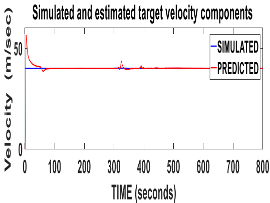
Fig.5 True and predicted velocity of target for scenario 2
