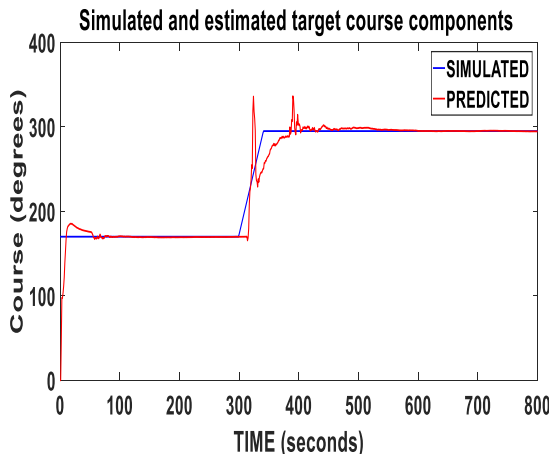
Fig.6 True and predicted course of target for scenario 2
