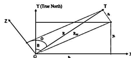
Fig.1.Target and observer positions
