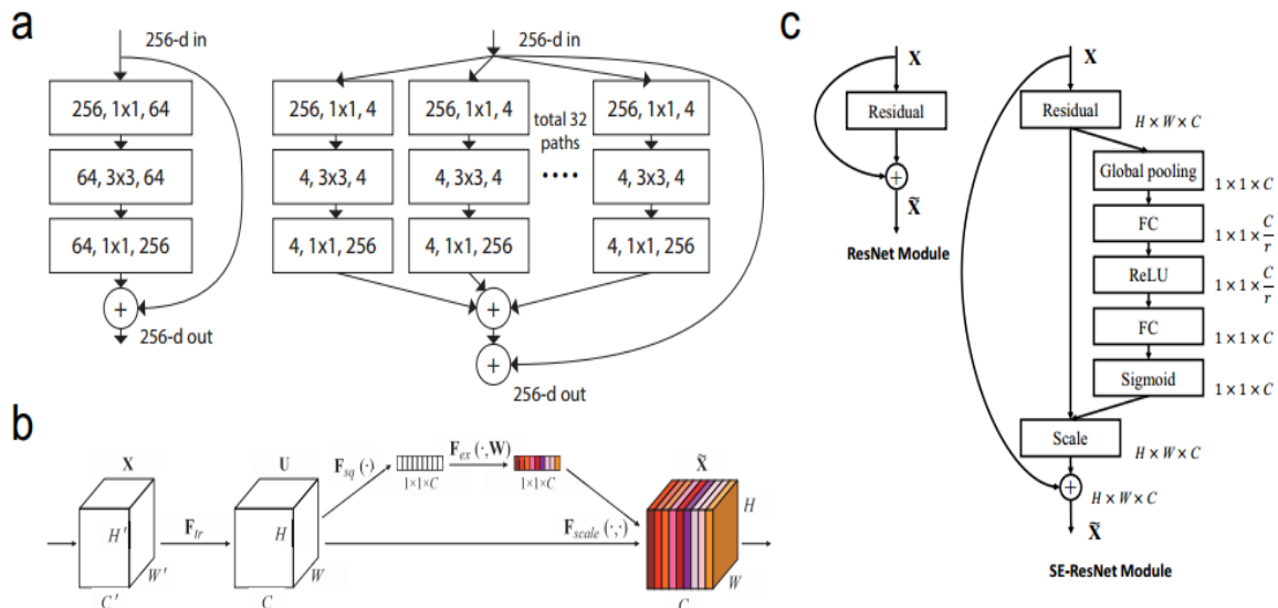
Figure 3. (a) The block of ResNet (left) and the block of ResNeXt with cardinality = 32 (right) [11].
