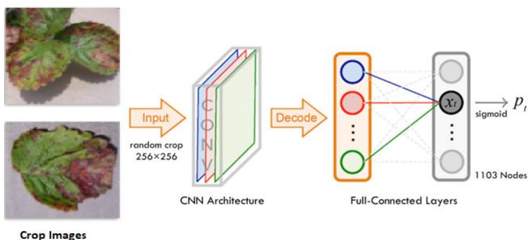
Figure 2. Schematic diagram of the CNN model, where the CNN architectures used in this work are ResNet-50, ResNet-101, and SE-ResNeXt-101 (32x4d)
