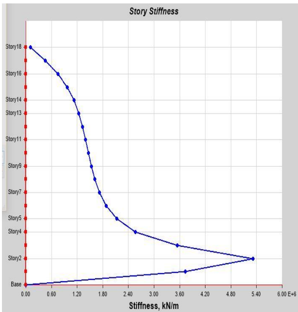
Fig -6 Storey stiffness- x axis- zone- iv
