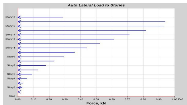
Fig -8 Shows ZONE III of base shear
