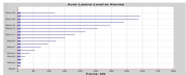
Fig -7 Shows ZONE III of base shear
