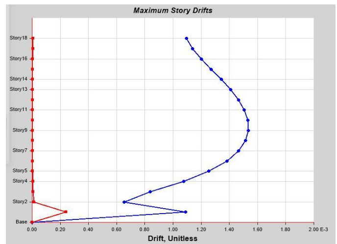
Fig no 4- Storey Drifts - ZONE IV
