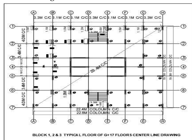
Fig no: 2 Centre line diagram of the building
