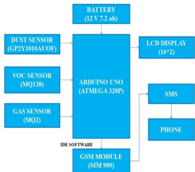
Fig 2.1 Block Diagram of Air Quality Monitoring System
