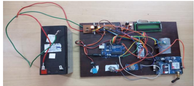
Fig 5.1 Interfacing of sensors with Arduino Uno
