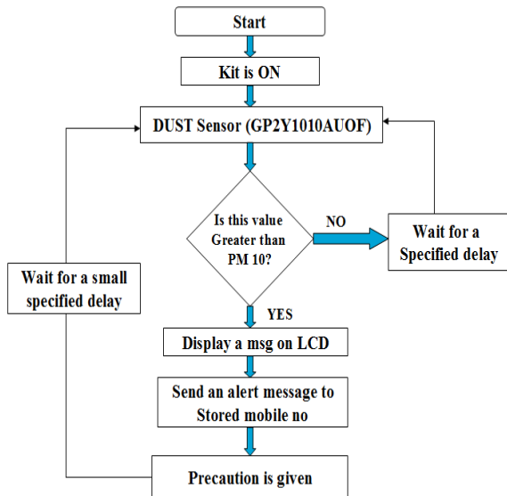
Fig 4.1.3 Flow chart of DUST Sensor using GSM
