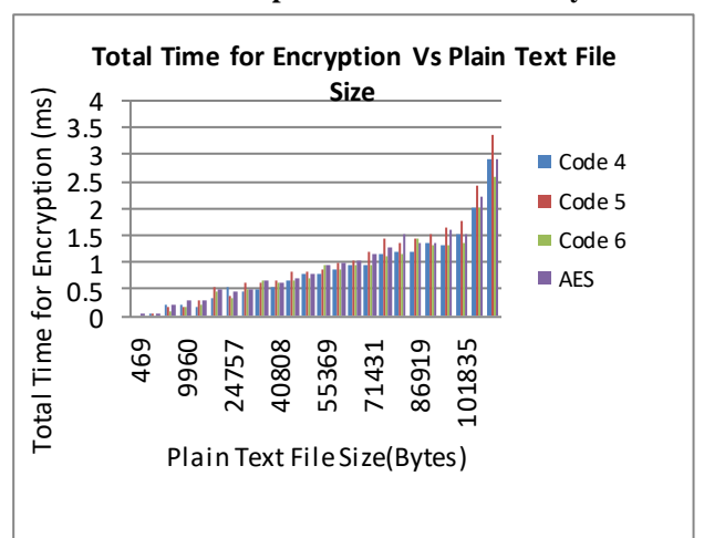
Fig.6: Total Time for Encryption and Plain Text File Size comparison for 2 dimension predetermine order key
