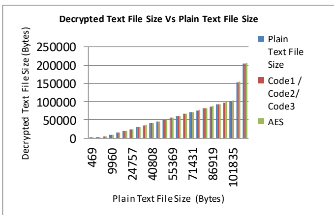
Fig.4: Decrypted Text File Size and Plain Text File Size comparison for 2-dimension predetermine order key Code1, Code2 and Code3 are the 2- dimension predetermine order key which generated by using 128 random numbers from 0 to 127.
