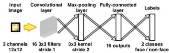
Fig.5 CNN Face detection
