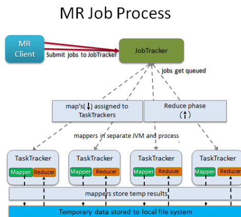
Figure 2: MapReduce Process
