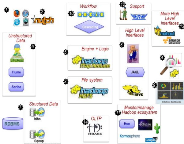
Figure 1: Hadoop Ecosystem
