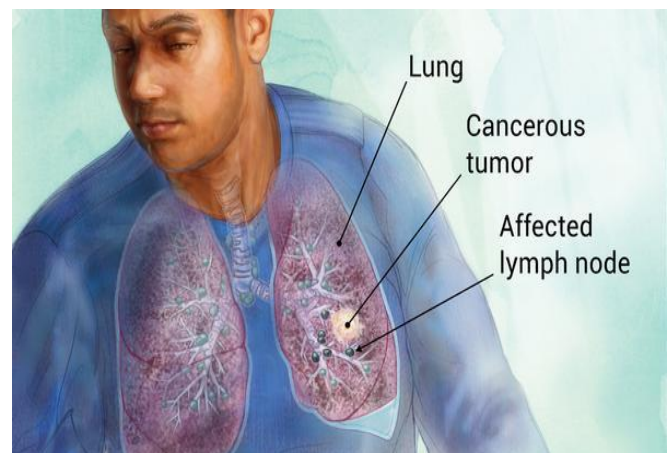
Fig. 1. Human Lung [3]
