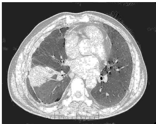
Fig.7. Histogram Equalization
