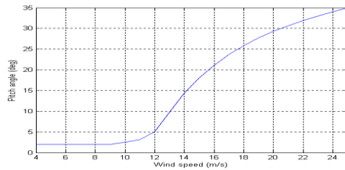
Fig. 4.6: Relationship between Pitch Angle and Wind Speed
