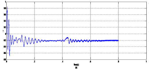
FIG 17 Simulation results with fuzzy logic controller methods of Torque under 5% voltage un balance and 1.2 p.u rotor speed
