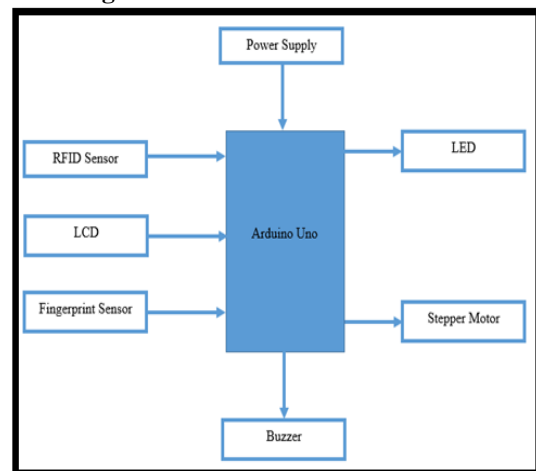
Fig. 3. Block diagram of Vehicle Door Security using Smart Tag and Fingerprint System
