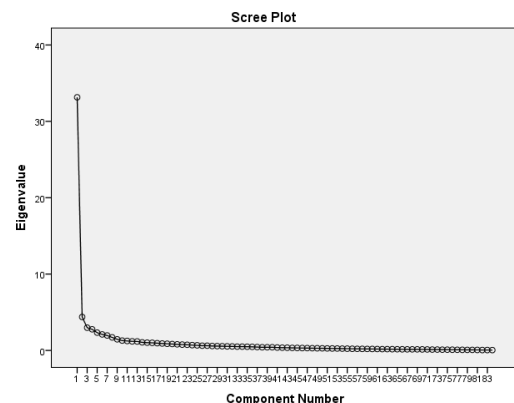
Figure 03 – Scree plot
