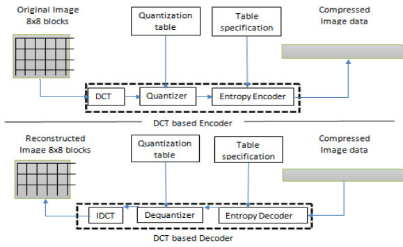
Figure 2: The block diagram of JPEG compression process
