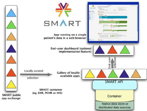
Figure 7: smart app
