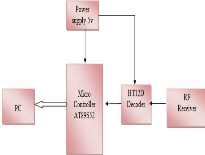
Fig 2. Receiver section B. Voice recognition kit using hm2007
