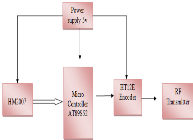
Fig 1. Transmitter section
