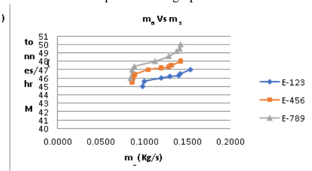
Figure1 mass flow rate of ash versus mass flow rate of air
