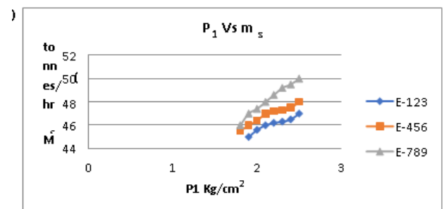
Figure2: Mass flow rate of ash versus inlet pressure
