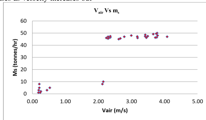
Figure 4 scatterplot of V air versus m s
