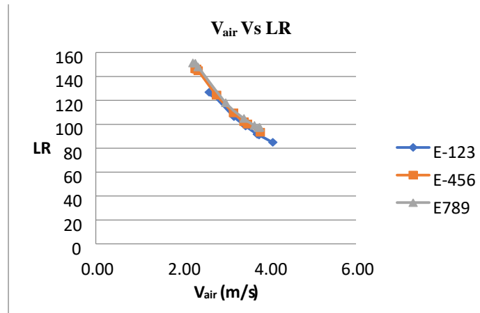
Figure3: V air versus Loading ratio
