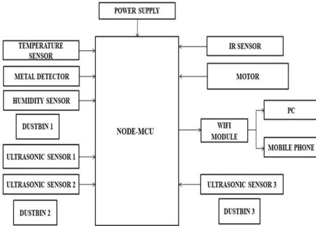
Fig. 2 Block Diagram
