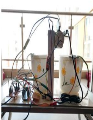
Fig. 5 Back View
