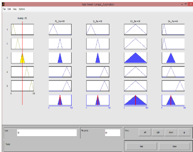
Fig 12 Rule viewer output
