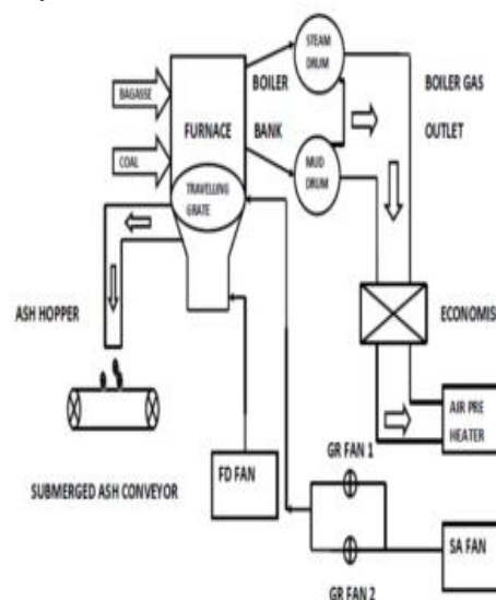
Fig 1 Furnace Operation
