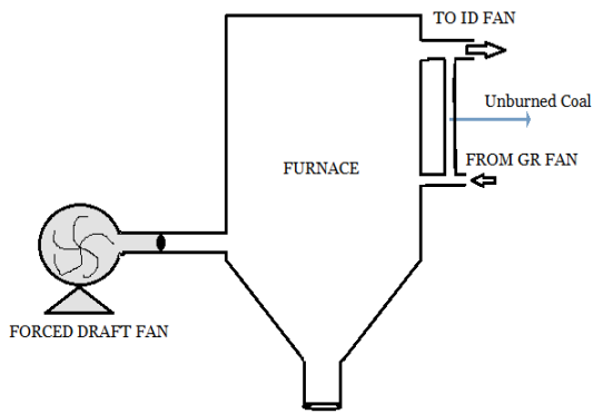
Fig 2 Forced Draft Fan[4]
