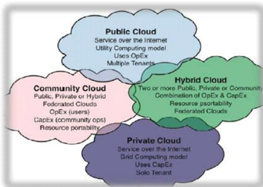
Figure 3: Cloud Model
