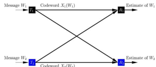
Fig. 2. Interference channels [6]
