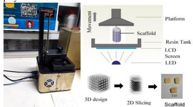
Fig. 2: The Machine Set Up for The DLP 3D Printing Process
