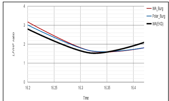
Figure V. Polar 7 and ECG calculated LF/HF ratio for Volunteer 7 data with three measurements
