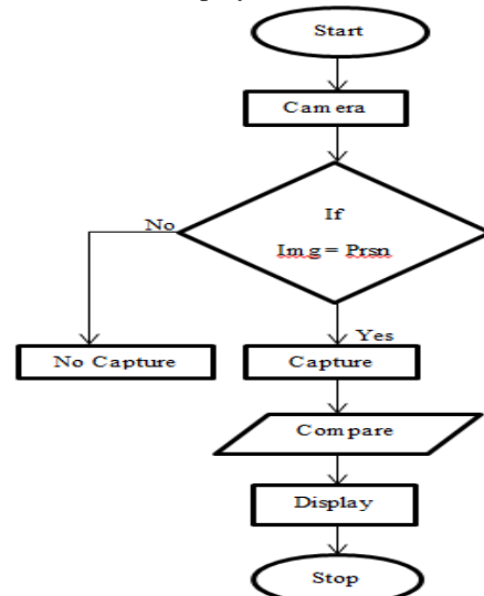
Figure3: Flowchart
