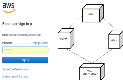
Figure2: Deployment Diagram
