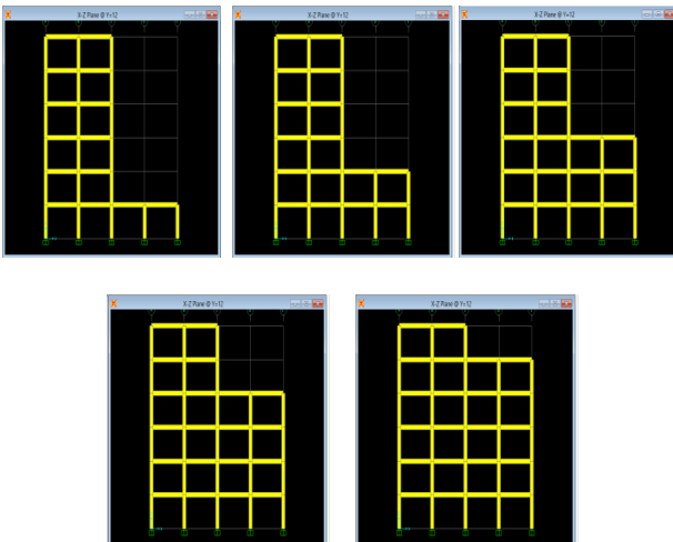
Fig. Model GI 1 to GI 5
