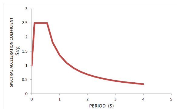
Fig. 7: Response Spectra for 5% Damping (IS1893:2002)
