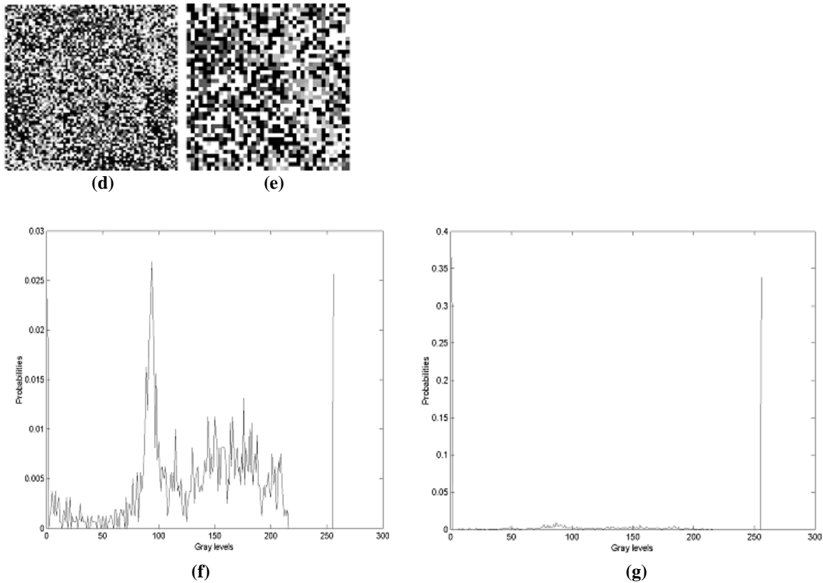
Figure 1. Impulse Noise Detection for the image Peppers with 5% and 70% of impulse noise. a) Original image(80X80),b) 5% impulse noise added image ,c) 1/4rth of image (b) with largest no. of midgray values(1064,first quadrant), d) 70% impulse noise added image, e) 1/4rth of image (d) with largest no. of midgray values (358), f) pdf plot of (c),g) pdf plot of (e).
