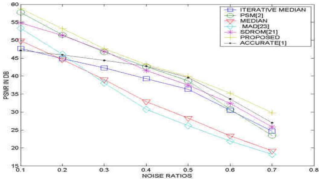
Figure 3 Average plot of Comparison of Different Noise Removal Methods on Different Test Images.
