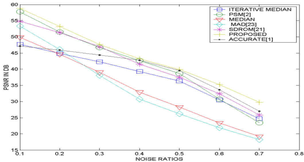
Figure 3 Average plot of Comparison of Different Noise Removal Methods on Different Test Images.
