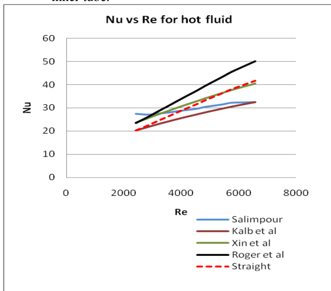
Fig. 5(a): Nusselt number vs. Reynolds number for hot fluid
