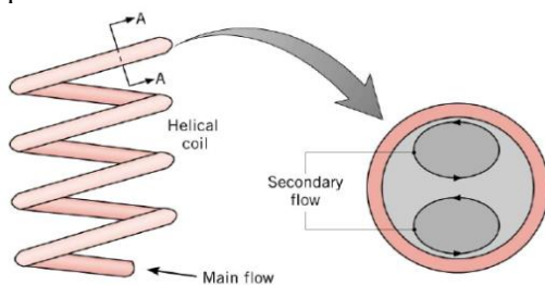
Fig.1. Secondary flow developed due to curvature
