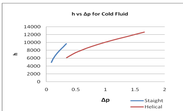
Fig. 7(b): heat transfer coefficient vs. pressure drop for cold fluid
