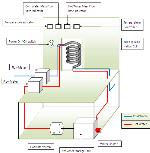
Fig.2. Schematic diagram of tube-in-tube helical coil heat exchanger experimental set-up
