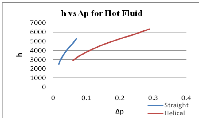
Fig. 7(a): heat transfer coefficient vs. pressure drop for hot fluid
