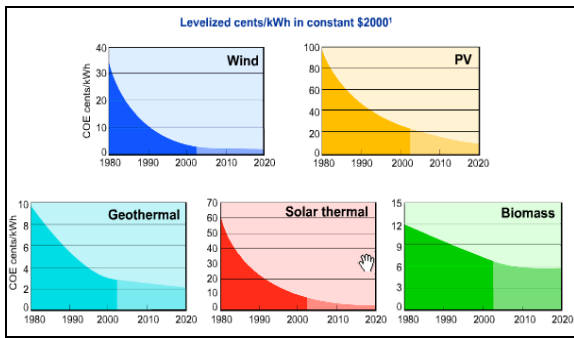
Fig 5. Renewable Energy Cost Trends.
