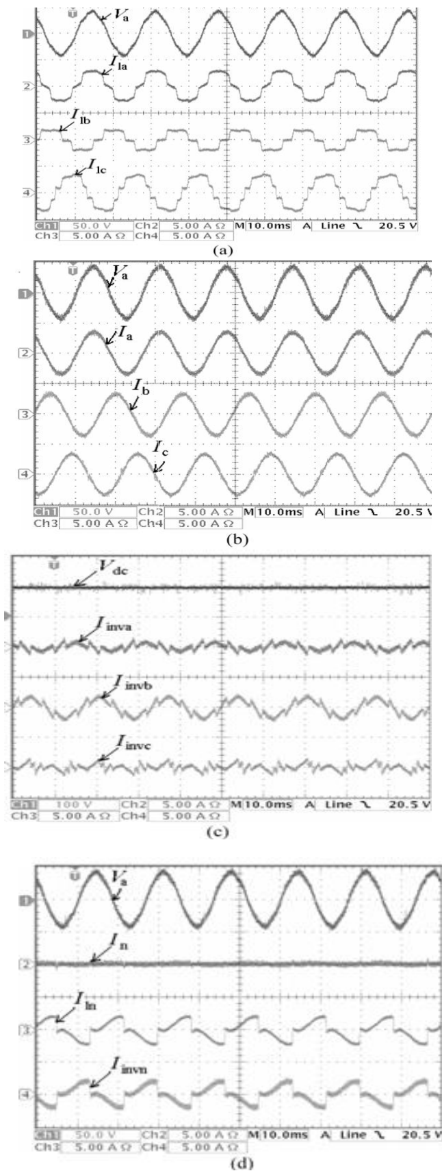
Fig. (6) Experimental results for the active power filtering mode ( P_{RES}=0 ): (a) unbalanced load currents, (b) grid currents after compensation, (c) currents injected by grid-interfacing inverter, (d) load, grid and inverter neutral currents.
