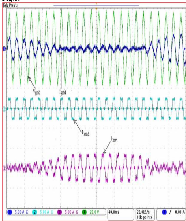
Fig.(8) Experimental results: Dynamic performance of proposed approach.
