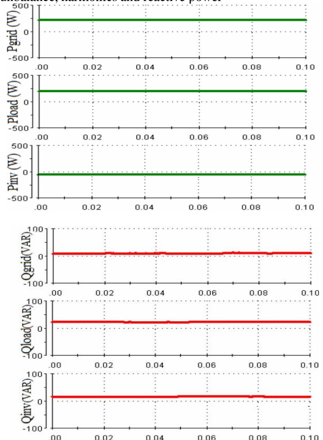
Fig. (7) Experimental results for the active power filtering mode ( P_{RES}=0 ) active and reactive power flow in real-time
