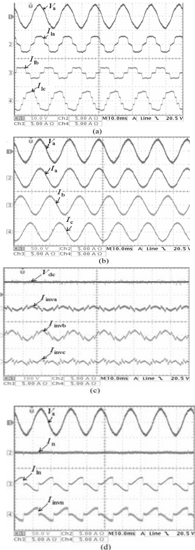
Fig. (6) Experimental results for the active power filtering mode ( P_{RES}=0 ): (a) unbalanced load currents, (b) grid currents after compensation, (c) currents injected by grid-interfacing inverter, (d) load, grid and inverter neutral currents.
