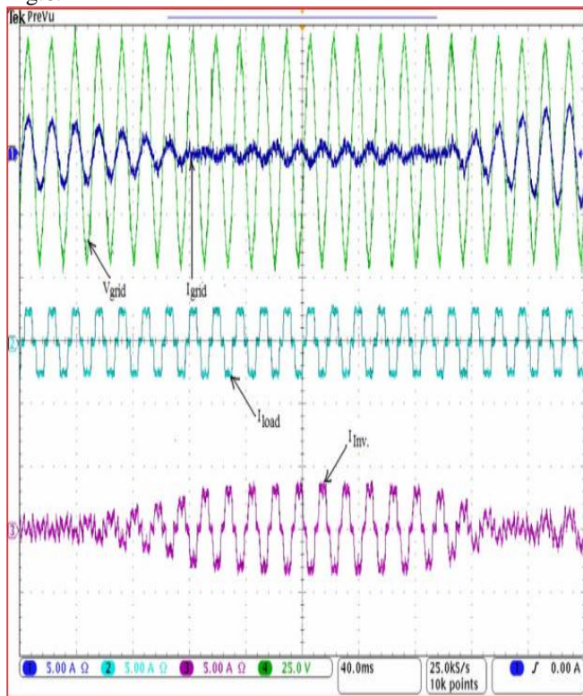
Fig.(8) Experimental results: Dynamic performance of proposed approach.
