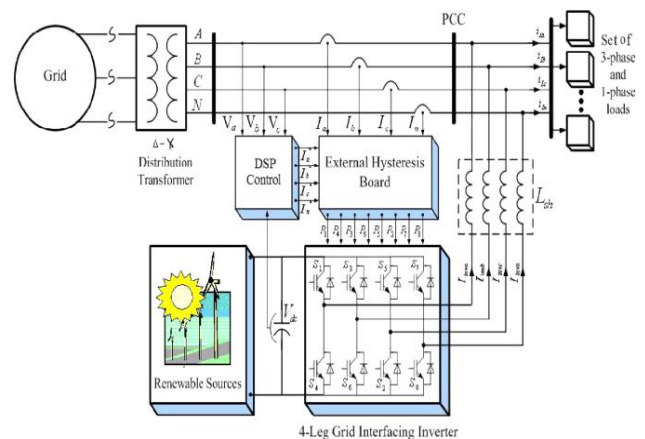
Fig.(1) Schematic of proposed renewable based distributed generation system
