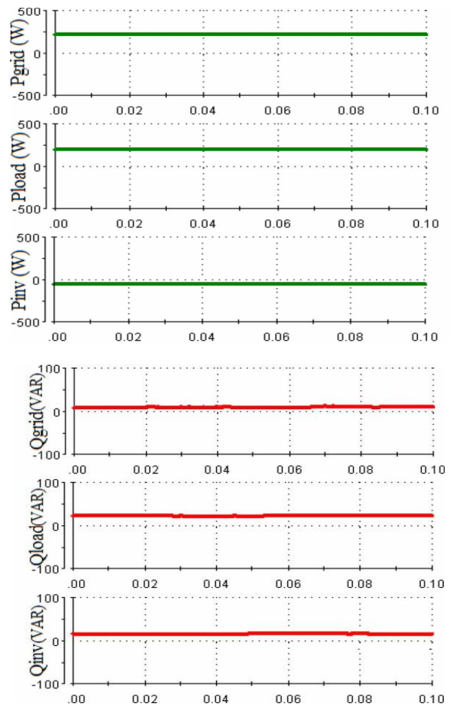
Fig. (7) Experimental results for the active power filtering mode ( P_{RES}=0 ) active and reactive power flow in real-time
