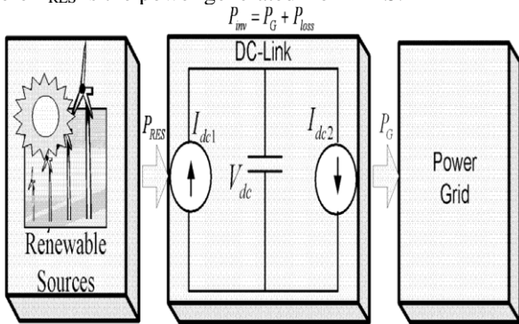
Fig.(2) DCLink equivalent diagram.
