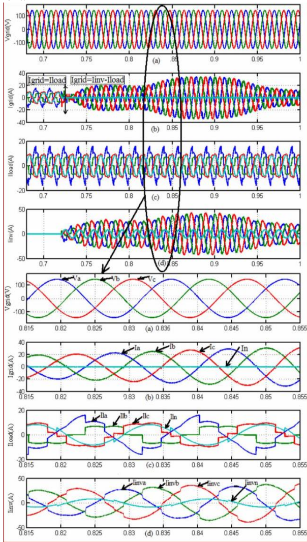
Fig. (4) Simulation results: (a) Grid voltages, (b) Grid Currents (c)Unbalanced load currents, (d) Inverter Currents.
