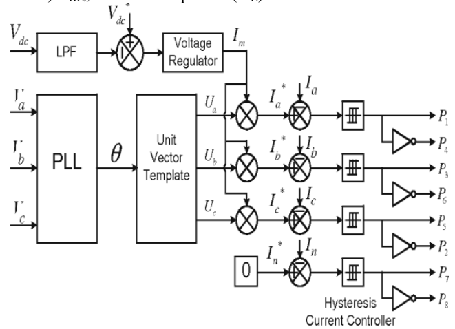
Fig.(3) Block diagram representation of grid-interfacing inverter control
