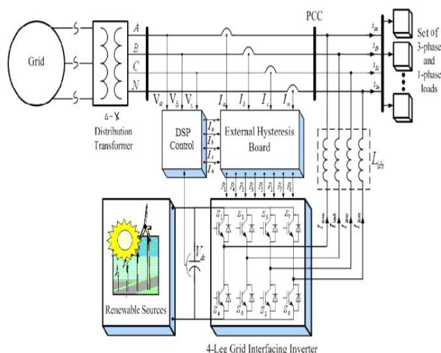
Fig.(1) Schematic of proposed renewable based distributed generation system
