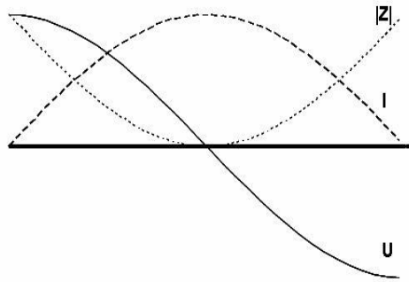
Voltage (U), current (I) and impedance (|Z|) distribution along the patch's resonant length
