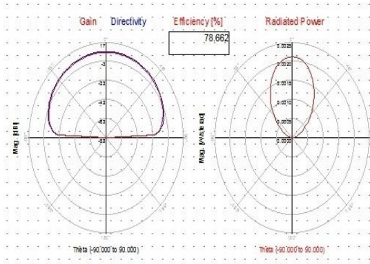
Fig. 5: Gain & Directivity plot
