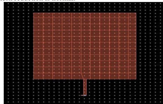
Fig.3: Meshed structure
