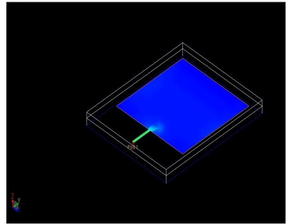
Fig. 9: Average current distribution with colour for the average strength of the current
