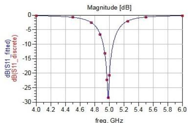
Fig. 4: Return Loss vs frequency plot
