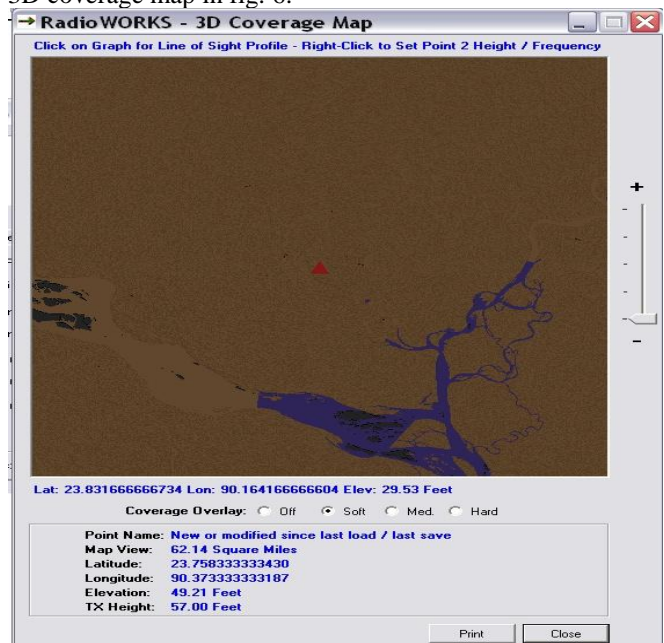
Fig. 6: 3D Coverage Map.
