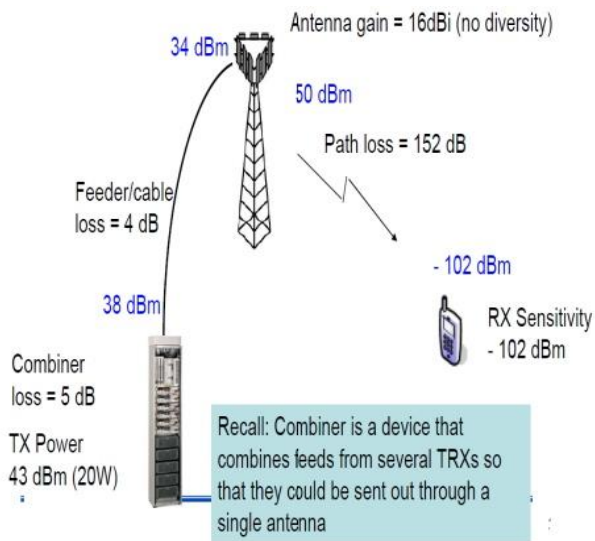
Fig. 5: Example of Link Budget Downlink Calculation.
