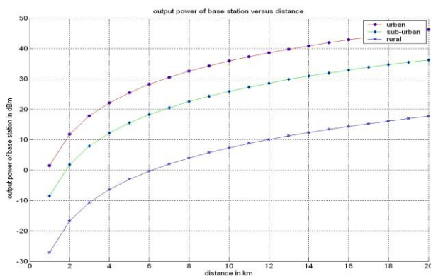
Fig. 9: Output Power of Base Station as a Function of Distance for Urban, Sub-Urban & Rural Area, at f=900\text{MHz} , h(r)=2\text{m} .
