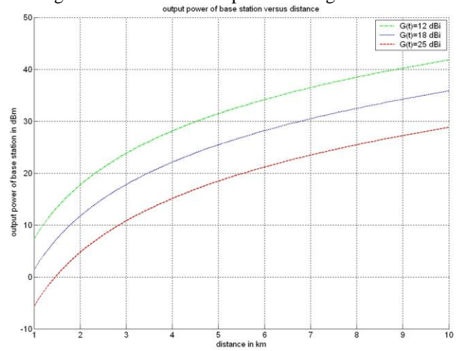
Fig. 10: Output Power of BS versus Distance for Urban Area at f=900\text{MHz} , h(r)=2\text{m} and G(t) Varied from 12 dBi to 25 dBi.
