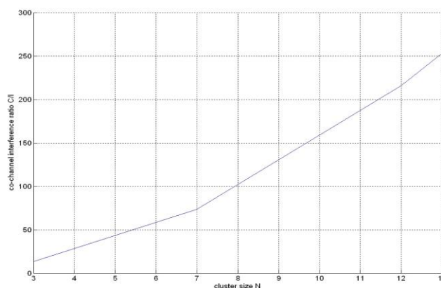
Fig. 3: Co-channel Interference Ratio versus Cluster Size.
