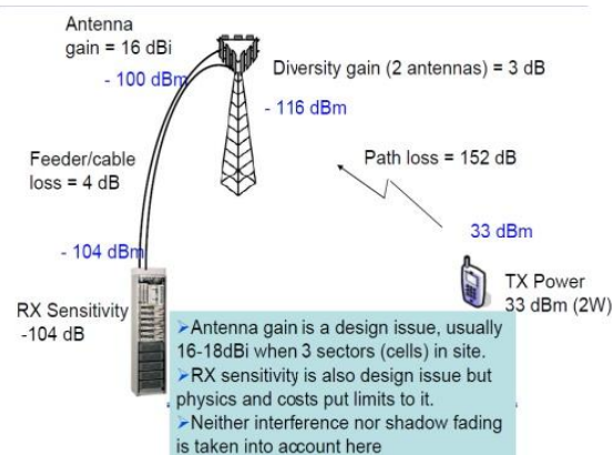
Fig. 4: Example of Link Budget Uplink Calculation.
